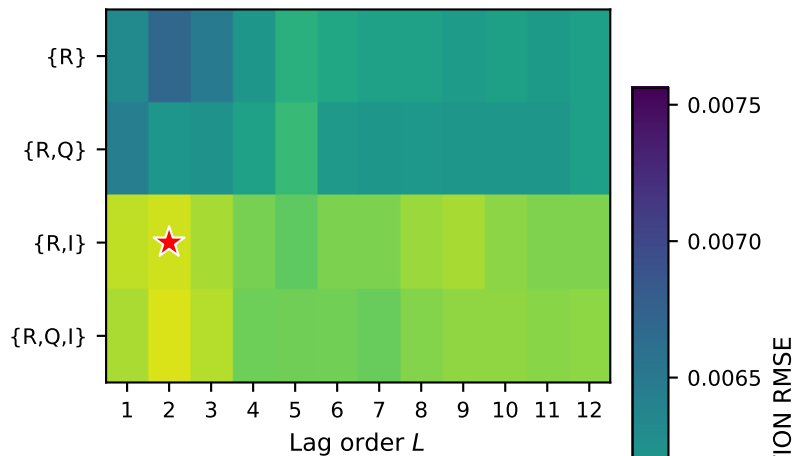
Transformer
