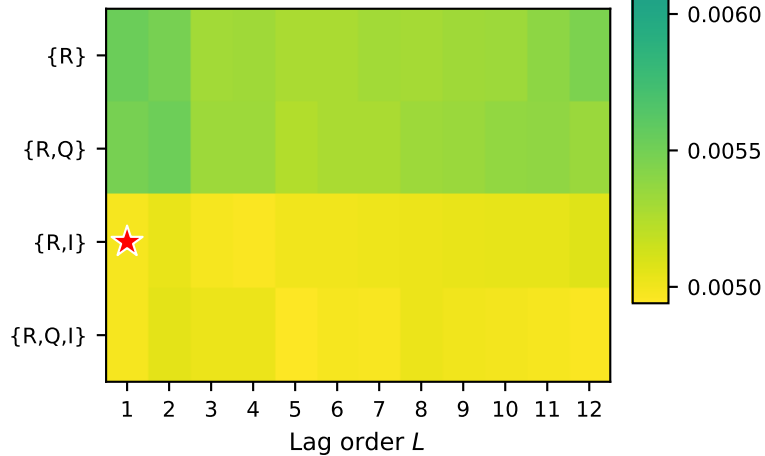
Transformer
